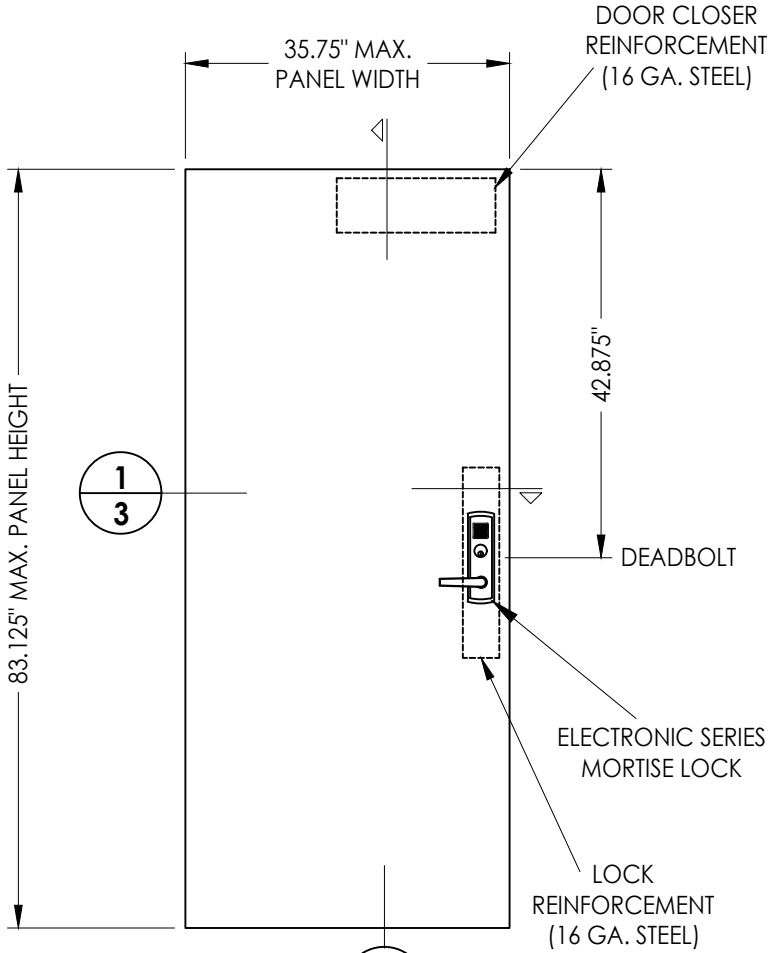
2 3 40 7'-0" STEEL DOOR PANEL (18 GA.) National Millwork Inc.
